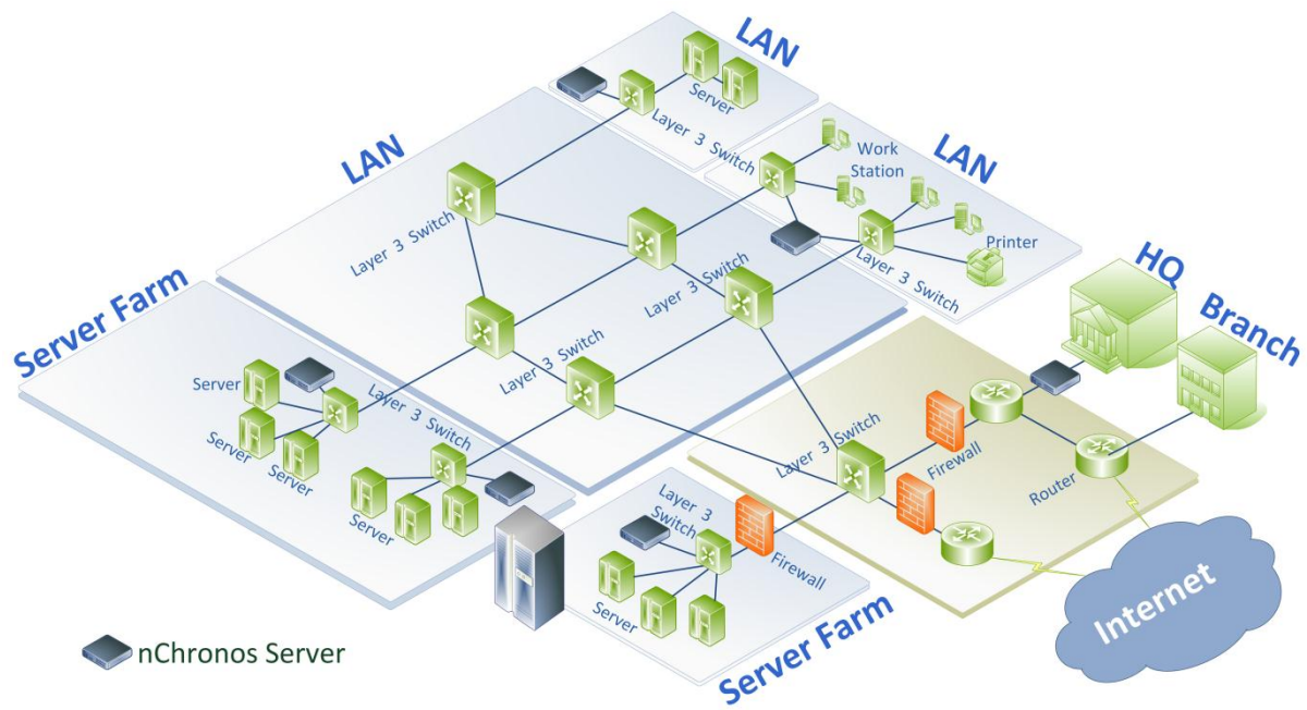
Figure 2 nChronos Deployment
